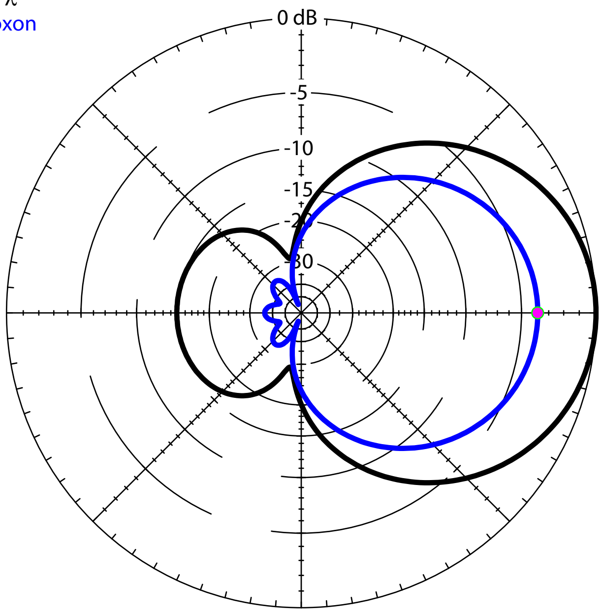
Single vs. Stacked Pair Moxons, Free Space
