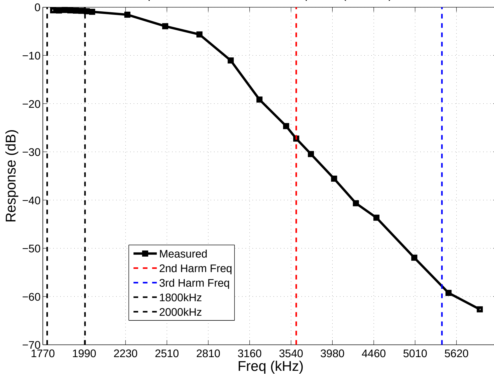
160m Diplexer Filter – Bare LPF Response (no HPF) – N3OX
